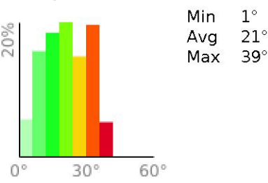
Slope Angle (top), Land Cover (middle), Tree Cover (bottom)
